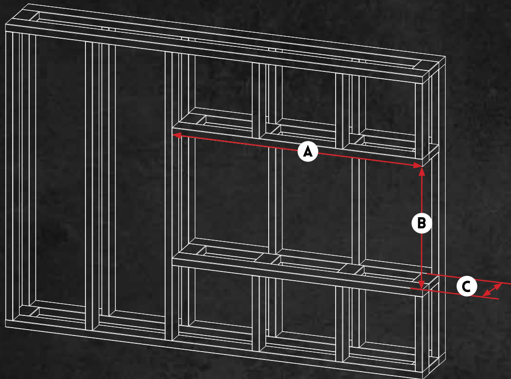
FINISHED WALL - THREE SIDED BAY INSTALL
